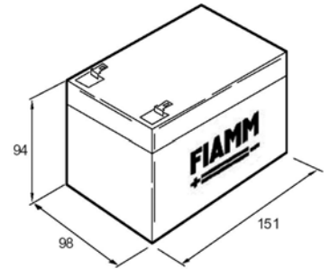
Battery dimensions (mm)
