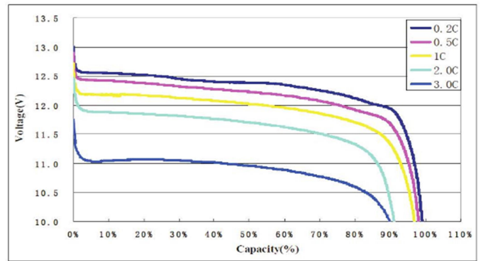
LVIF – 12,8V LiFePO4 LIVEN Battery Different Rate Discharge Curve (25°C)
