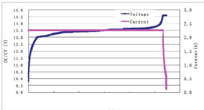
LVIF – 12,8V LiFePO4 LIVEN Battery Battery Charge Curve (0,2C; 25°C)
