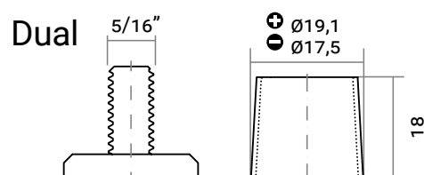
DT (Dual Terminal - Post & Stud)
