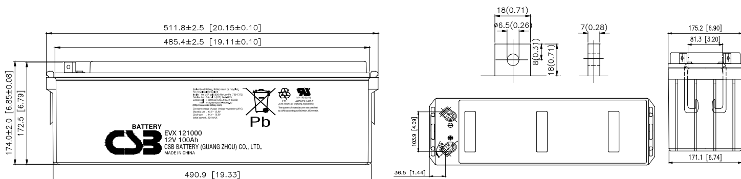
A Detail Drawing
