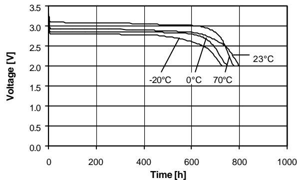
Temperature performance Load 12kW
