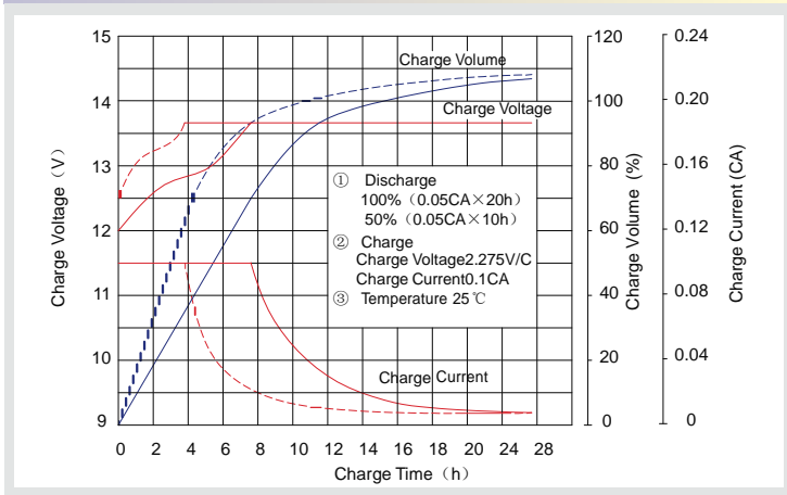
Charge characteristic: GUV for standard use
