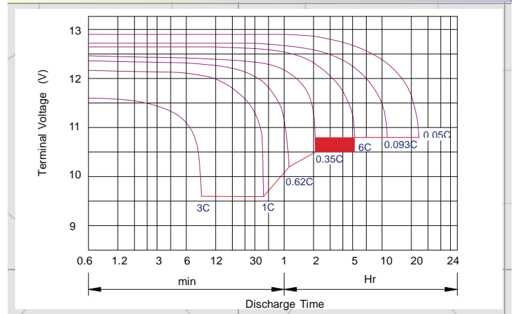
Discharge characteristic: GUV
