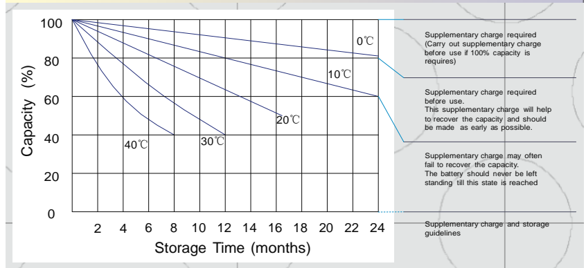
Storage characteristic
