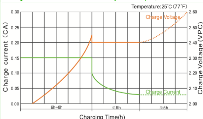
Charge Characteristic Curve For Cycle Use (IUI)
