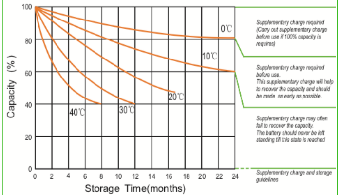
Storage Characteristics
