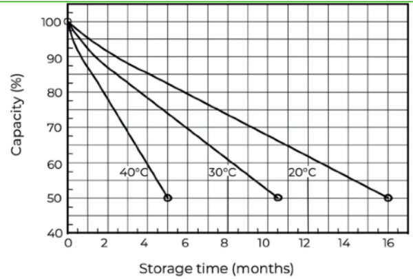
Storage Characteristics
