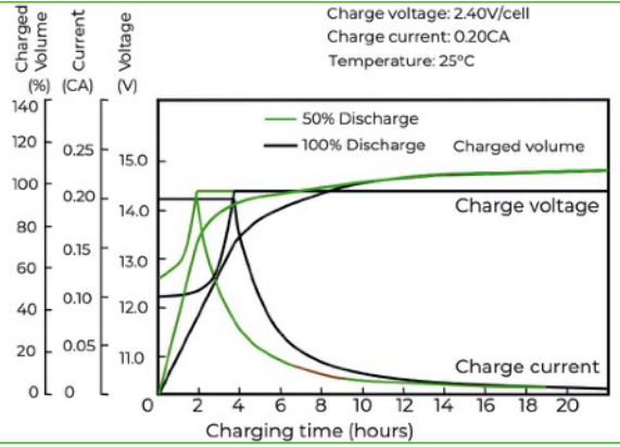
Charging Characteristics
